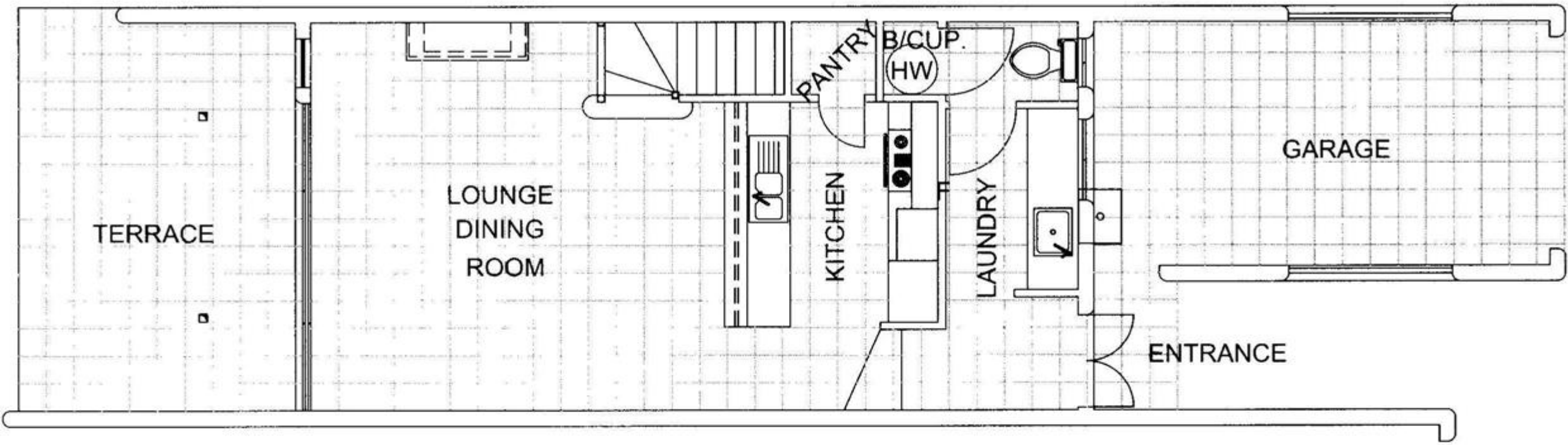
GROUND FLOOR
