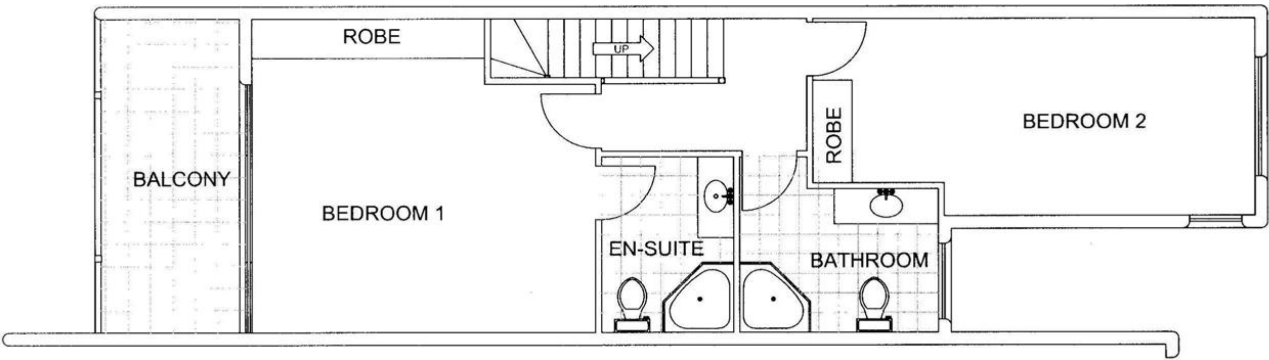
FIRST FLOOR
