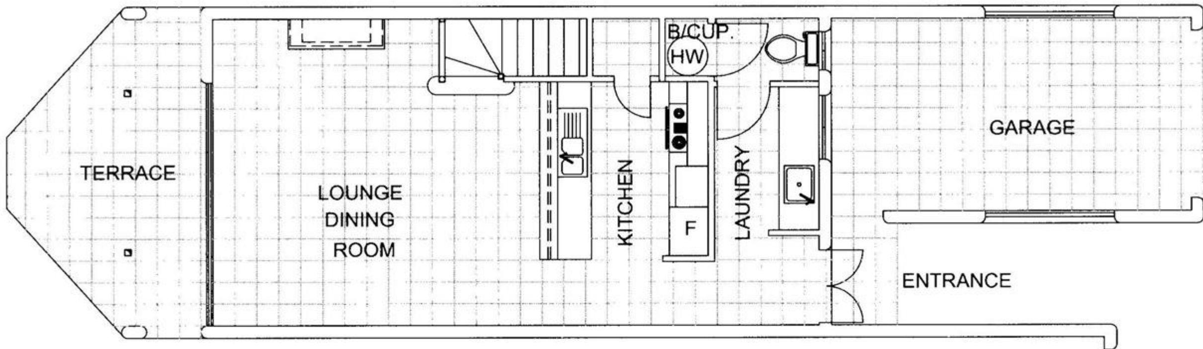
GROUND FLOOR
