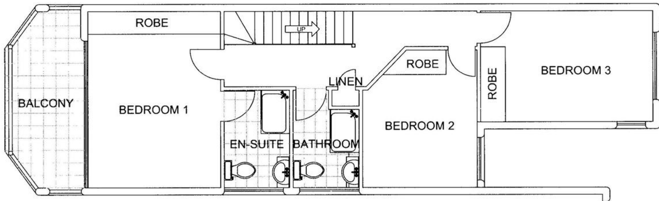
FIRST FLOOR
